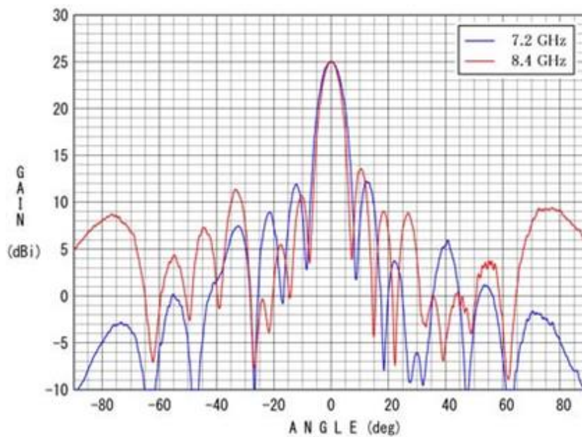
Typical Radiation Pattern
