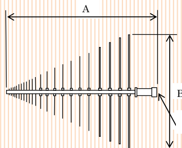
LP-0821, LP-2021 Outline View
